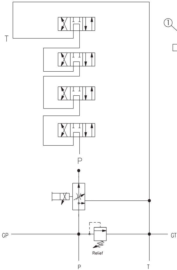
HYDRAULIC SCHEMATIC
